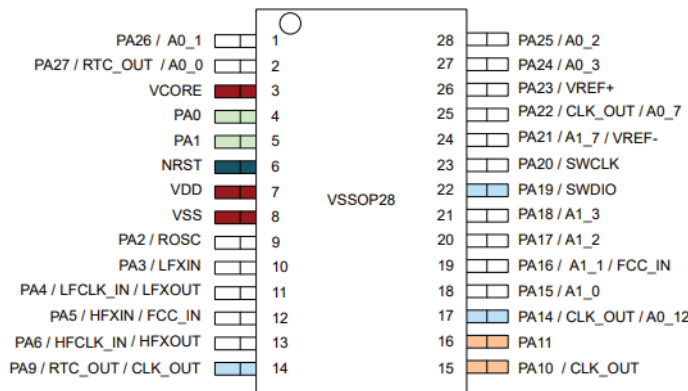
Figure 6-6. 28-Pin DGS28 (VSSOP) (Top View)
